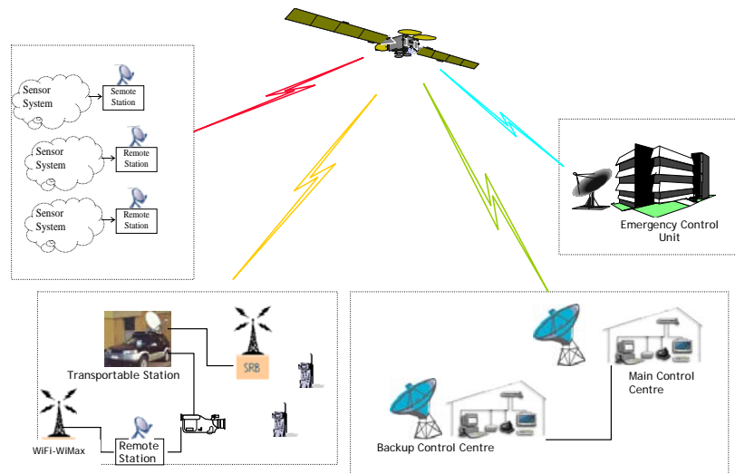
Figure 1 Communication Network Block Diagram
